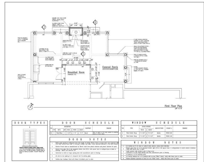
Proposed First Floor Plan Details showing material to be used
